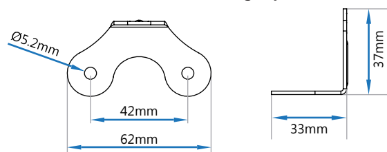
Mounting Clip
